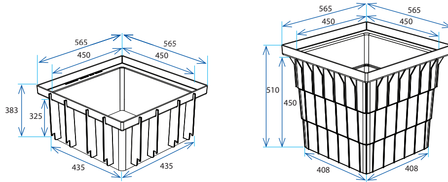
Series 450 Shallow Stormwater Pit
