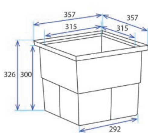
Series 300 Shallow Stormwater Pit
