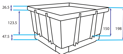
Series 300 Riser
