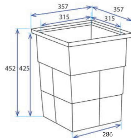
Series 300 Deep Stormwater Pit
