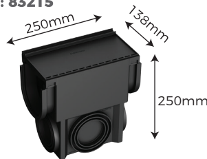
EasyDRAIN™ Edge Access Pit & Grate EI code: 83215
