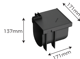
EasyDRAIN™ Edge Internal Corner & Grate EI code: 83220
