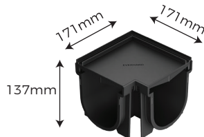
EasyDRAIN™ Edge External Corner & Grate EI code: 83225
