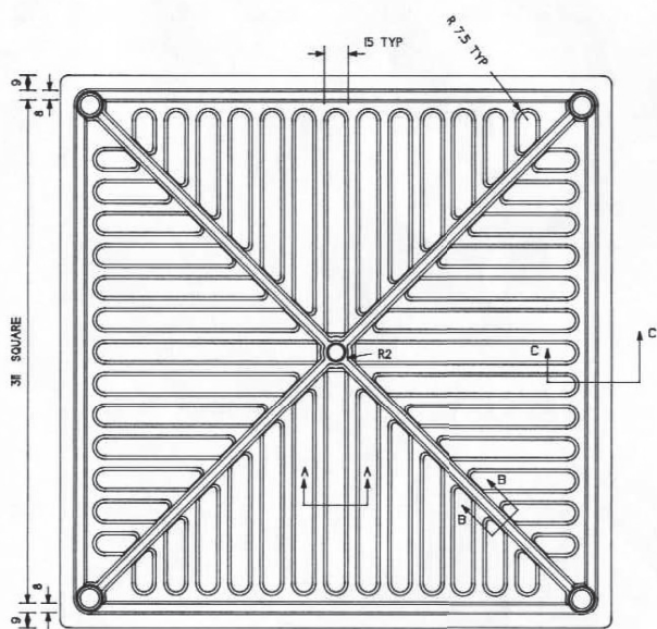
UNDERSIDE VIEW
