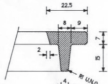
SECT CC
