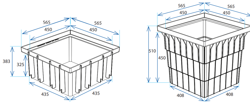
Series 450 Shallow Stormwater Pit
