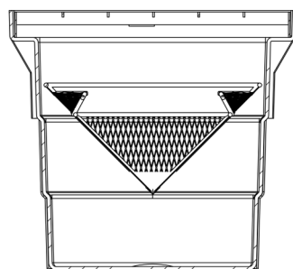
SECTION C-C SCALE 1 : 6
